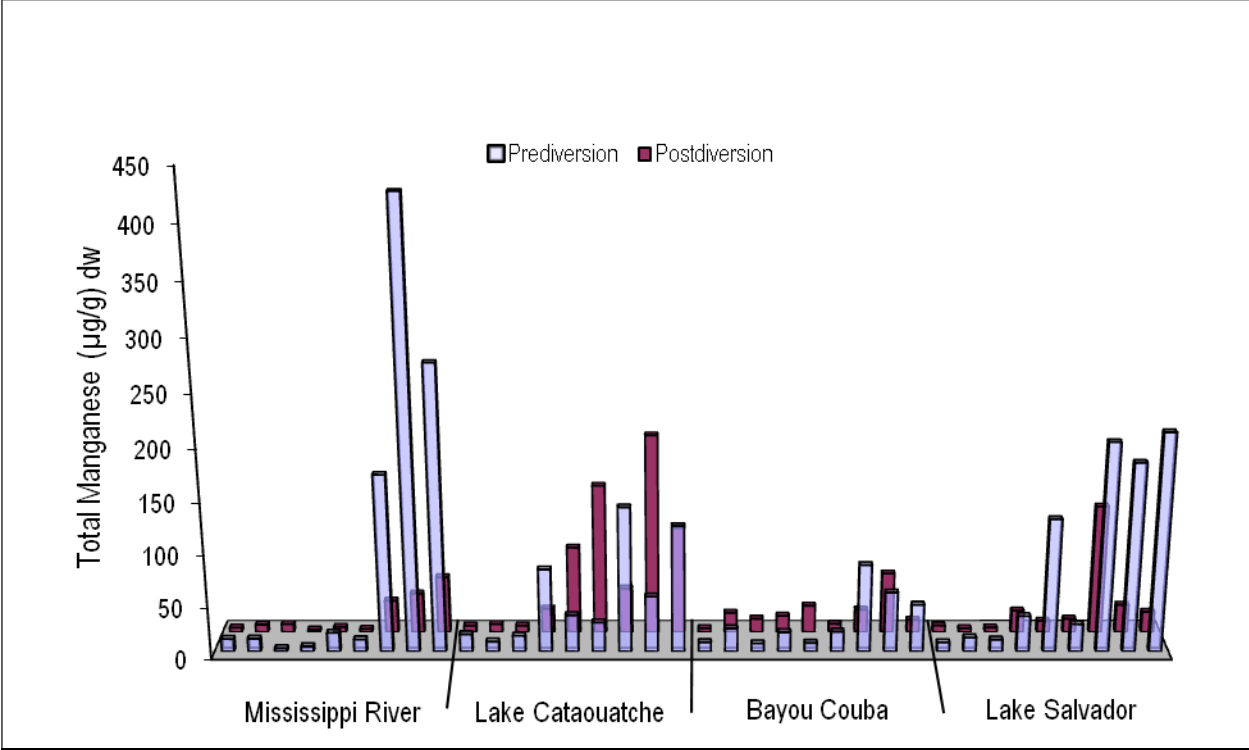
Figure 19B. Three-dimensional comparison of Davis Pond prediversion and postdiversion values for manganese by dry weight (in micrograms per gram [ \mu\text{g/g} ]).
